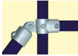
TYPE I74 SWIVEL STEP CROSS SIZE 4 ONLY
